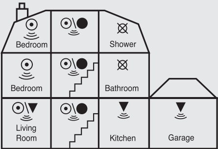
Multi Storey Dwelling LD1
