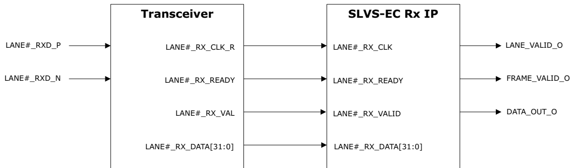
Figure 1 • SLVS-EC IP Block Diagram
