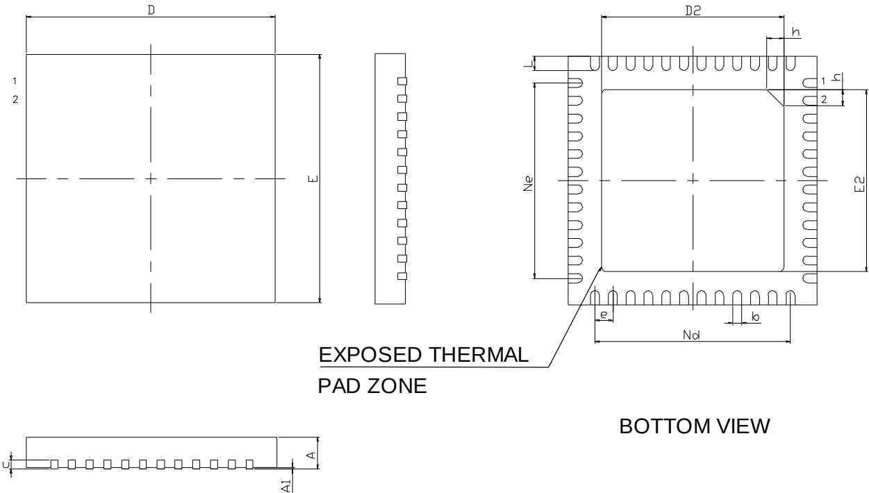
Figure 4-1 Package Outline QN48
