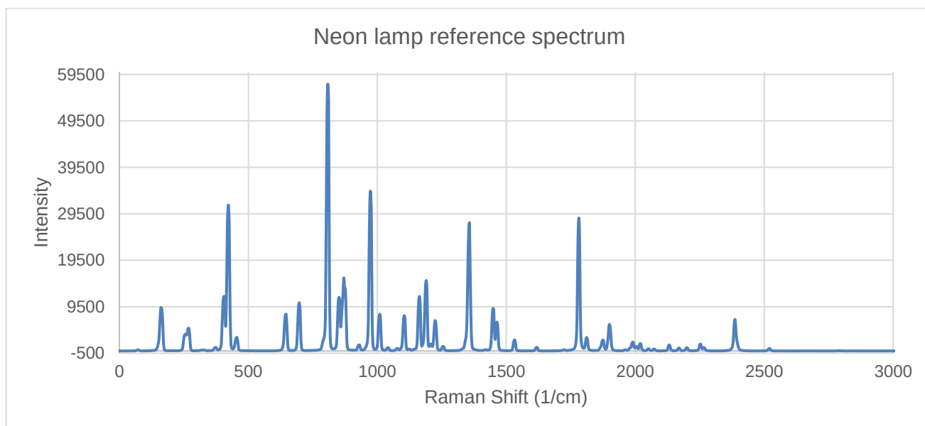
Figure 16. Neon light reference spectrum plotted in Raman wavenumbers (not wavelengths).
