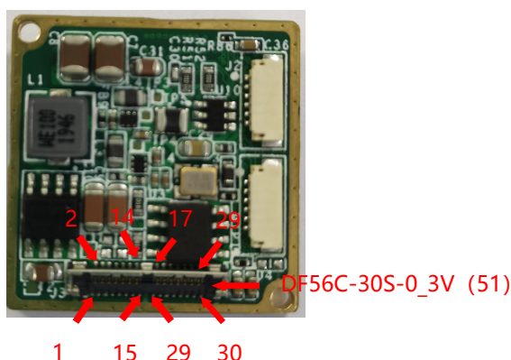
Figure 5.1 MRIII00V110F017C Expansion Board
