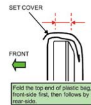
SET COVER
