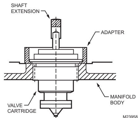
Fig. 3. Installation
