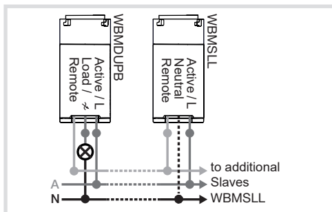
Fig. 5: 2 way connection
