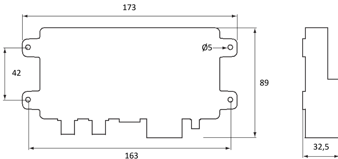
Figure 4.1: Dimensions
