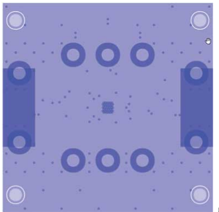
Figure 5. ADCA5190-EVALZ Assembly Drawing (Bottom Side, No Components)
