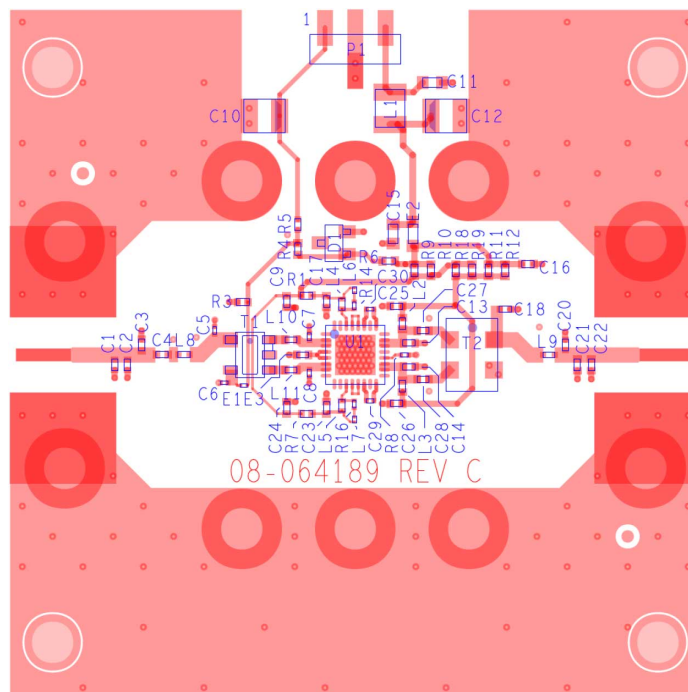
Figure 4. ADCA5190-EVALZ Assembly Drawing (Top Side)
