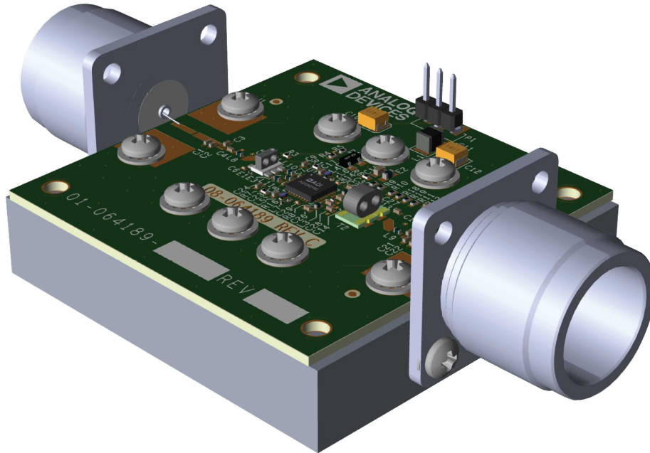
Figure 6. ADCA5190-EVALZ Top Side, Fully Assembled
