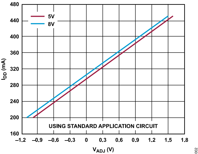
Figure 2. I_{DD} vs. V_{ADJ}
