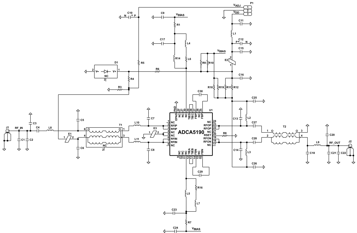
Figure 3. ADCA5190-EVALZ Evaluation Board Schematic
