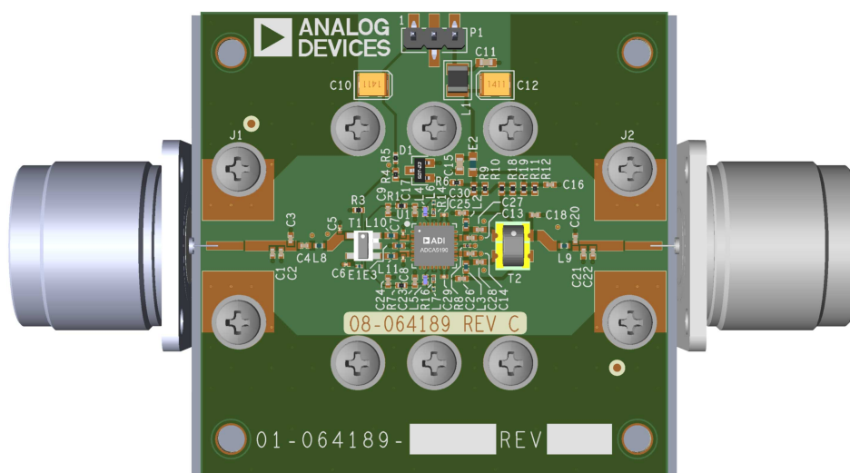
Figure 1. ADCA5190-EVALZ Photograph (Top Side)
