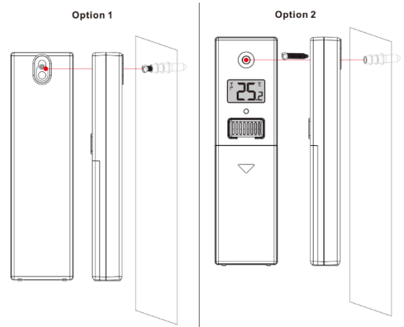
Installation method 1
