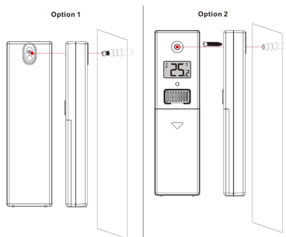
Installation method 1
