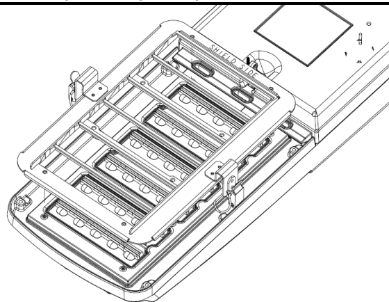
Figure 1 – Light Trespass Shield, Pre-Installation
