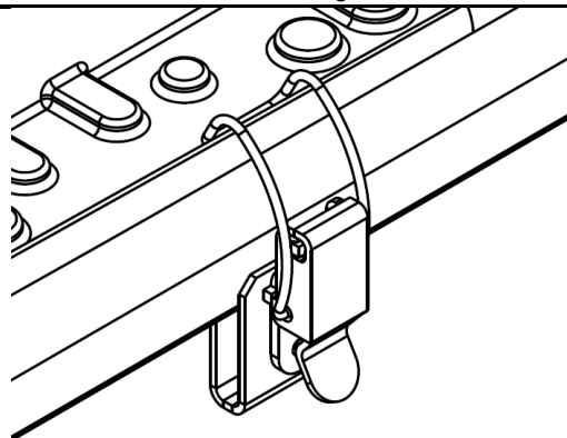
Figure 2 – Shield/latch Installed
