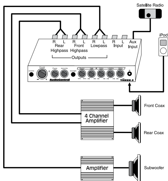
Figure 7: The THREE.2 can be mounted into a boat or RV and iPod can be a removable source unit
