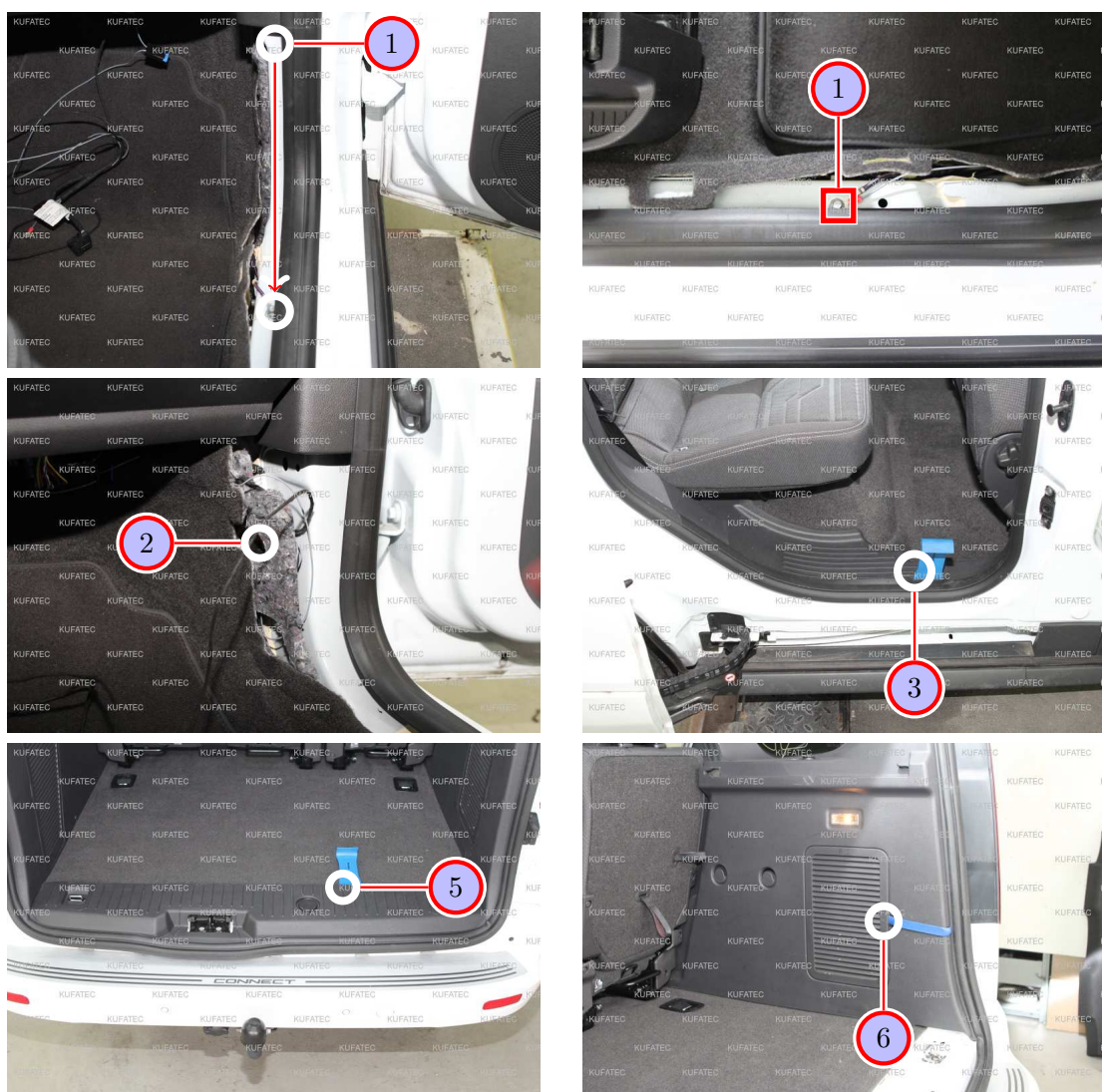
Figure 6: Connection ground / Removing trim panel rear
