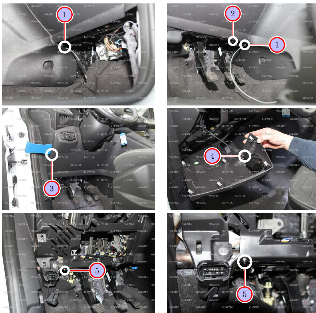
Figure 9: Installation pushbutton
