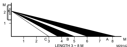
Fig. 1. Side view of PIR detection pattern.
