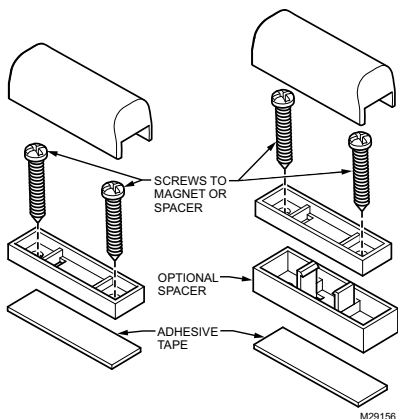
Fig. 10. Door magnet mounting options.
