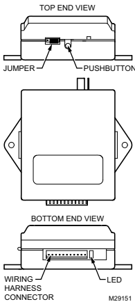
Fig. 5. Receiver components.
