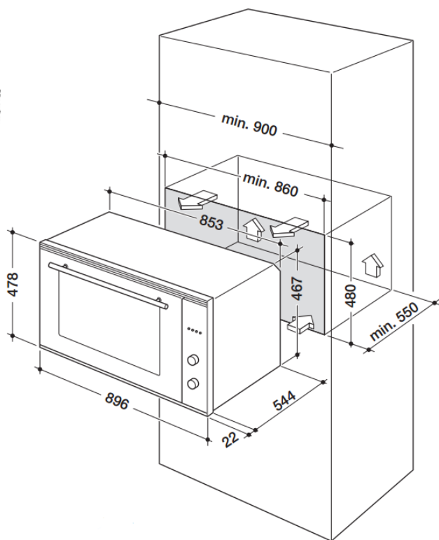
Column Installation
