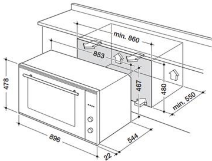
Base Installation
