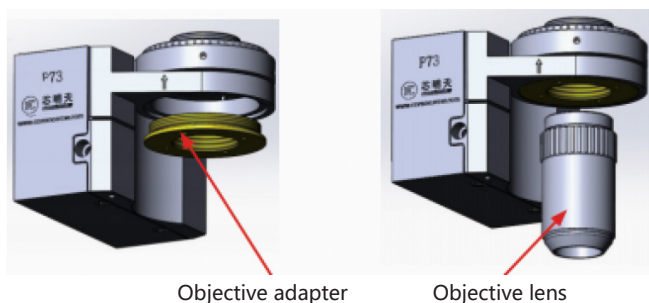
FIG.2 Installation diagram
