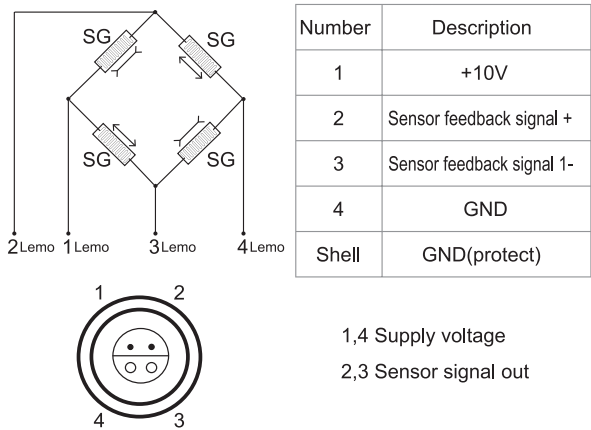
FIG.8 Definition of Sensor Connector
