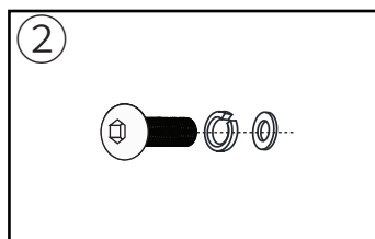
2 Bolts M8x25mm Quantity: 20
