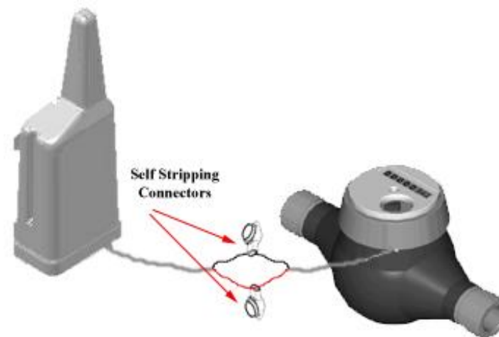
Figure 4: Wiring
