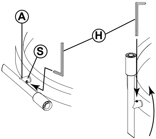
Drawing 3 - Assembly
