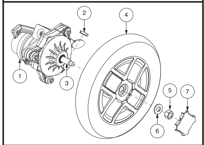
Figure 13. Drive Wheel Removal
