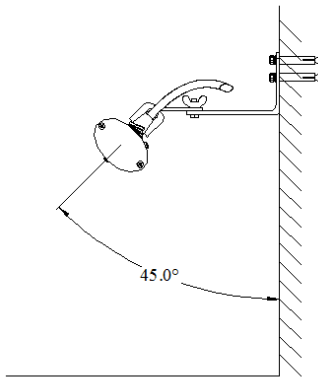
Figure3: Tilt angle.
