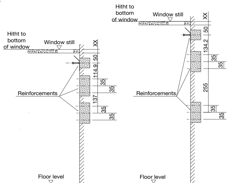
Figure 1. Dimensions for the strengthening of the wall.
