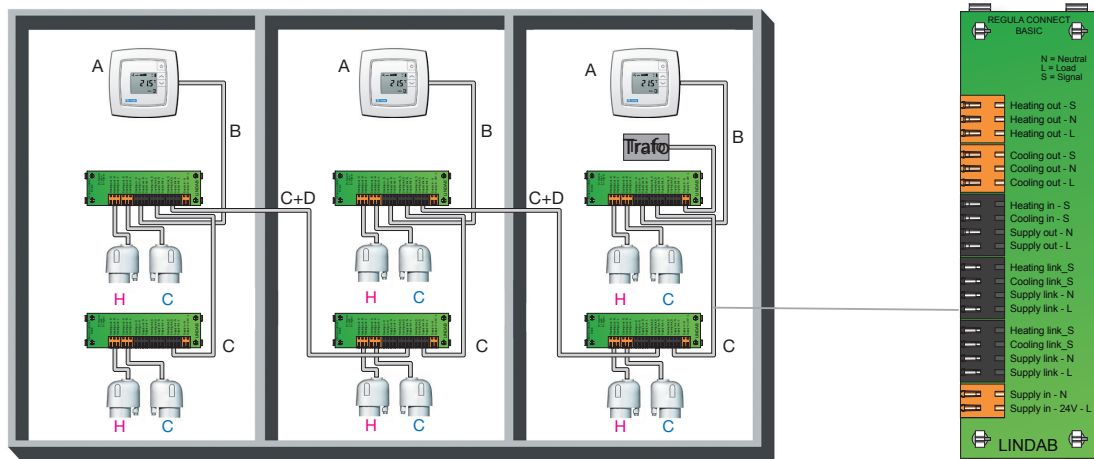
Figure 6. Connection card.
