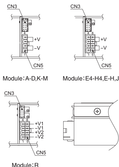
Fig. 6.1 Example of -J2 option
