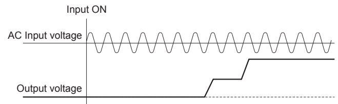
Fig.2.1 Start-up waveform in series and parallel operation
