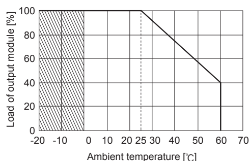
Fig. 6.3 Derating curve for ambient temperature (-F3 option)
