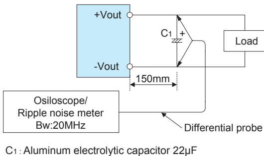
Fig.3.1 Measuring method of Ripple and Ripple Noise
