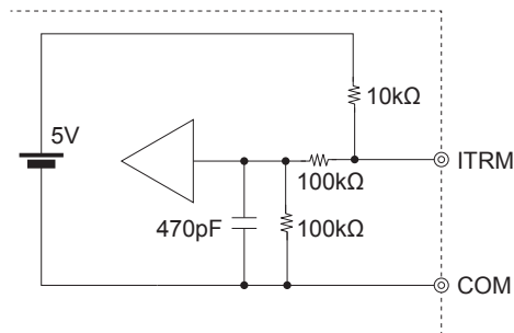
Fig.3.4 ITRM Internal circuit
