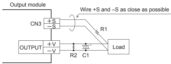
Fig. 3.6 Use example of remote sensing
