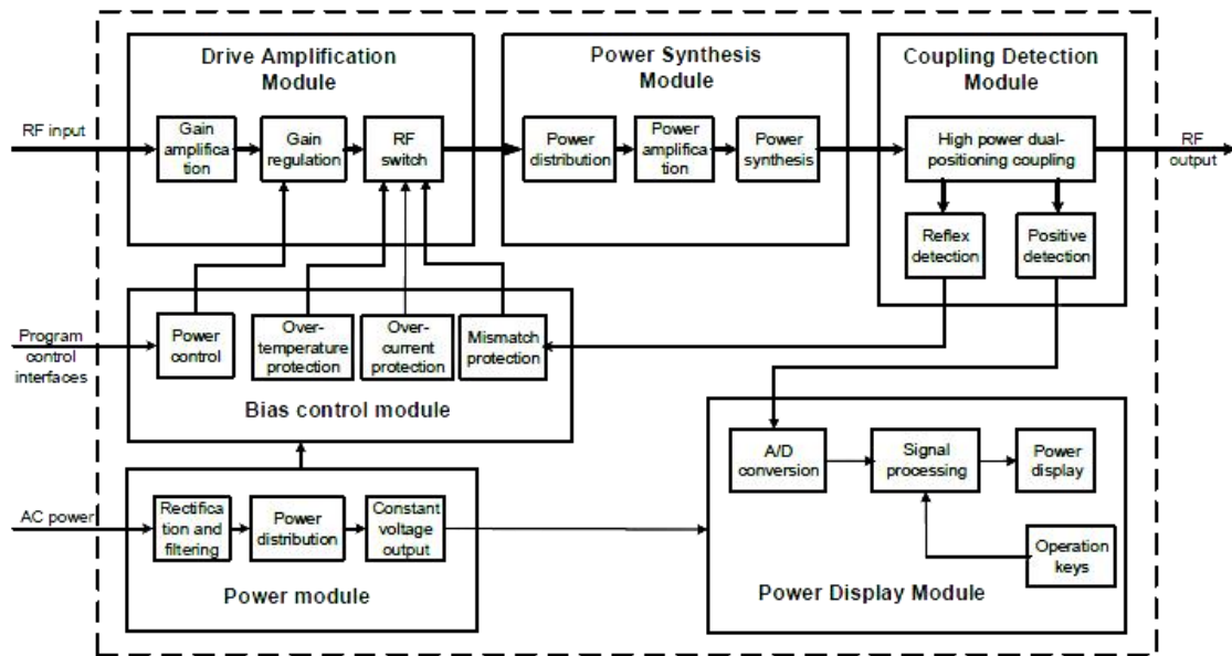
Figure 4-1 Schematic diagram for amplifiers of S3871 series solid-state power amplifiers
