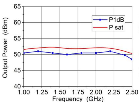
S3871AA Output power VS Frequency
