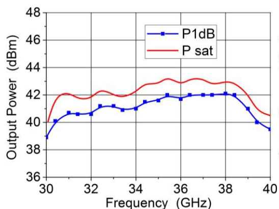
S3871FB Output power VS Frequency
