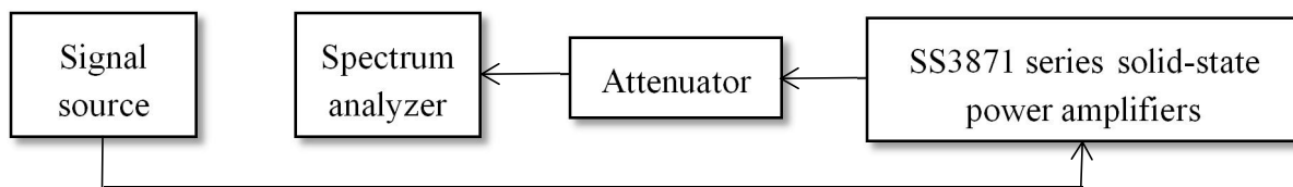
Figure 5-3 Diagram of the non-harmonic suppression test
