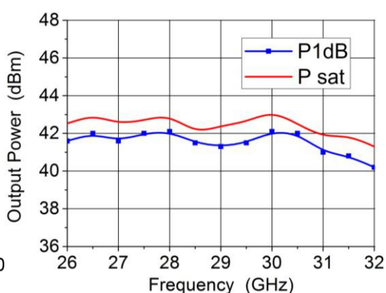
S3871FA Output power VS Frequency
