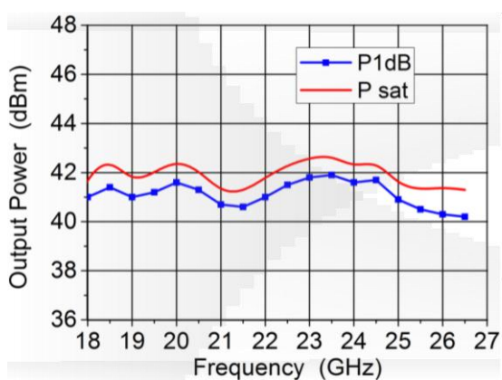
S3871EA Output power VS Frequency
