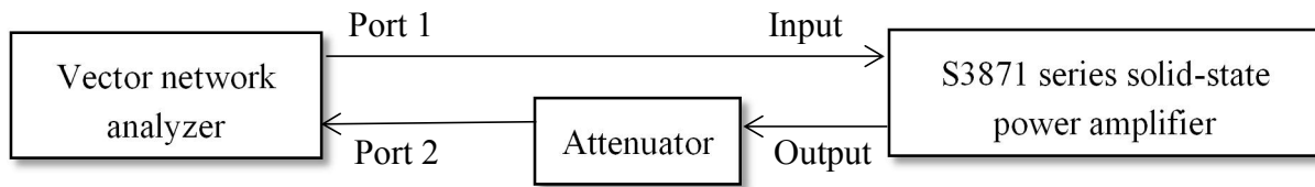
Figure 5-1 Gain and standing wave testing diagram
