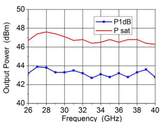
S3871FF Output power VS Frequency
