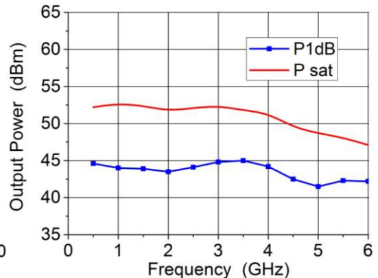
S3871AB Output power VS Frequency
