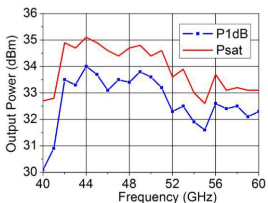
S3871LA Output power VS Frequency
