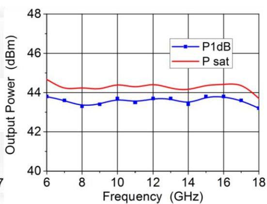
S3871DA Output power VS Frequency
