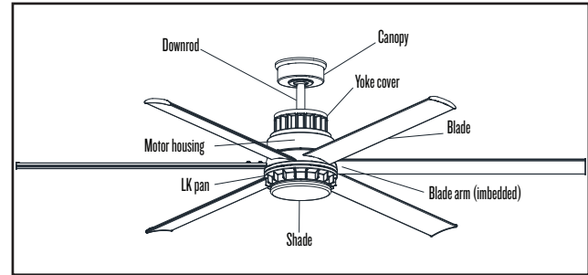
Parts identification on assembled fan.
