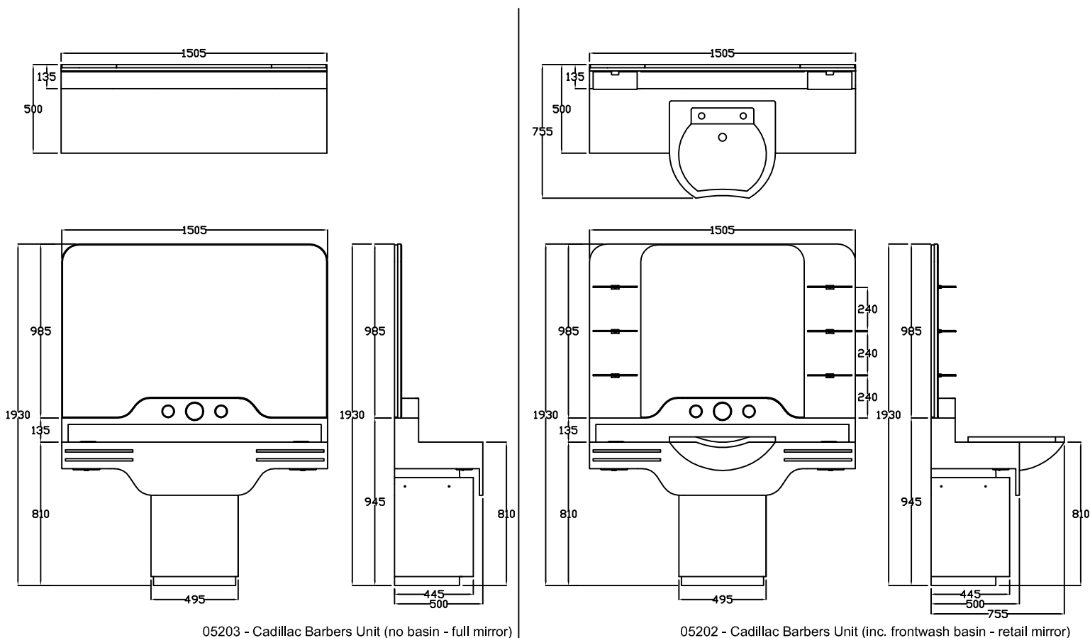
05203 - Cadillac Barbers Unit (no basin - full mirror)
