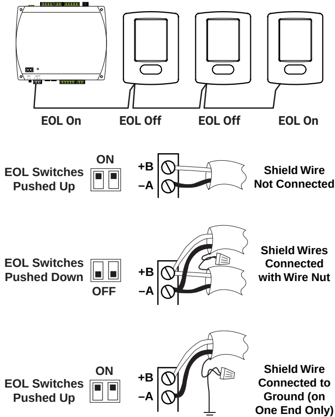
Illustration 10—MS/TP Connections and EOL (MS/TP Models)
