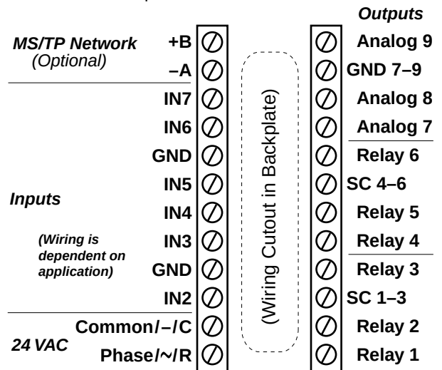
Illustration 5—BAC-19xx63 Terminals and Connections
