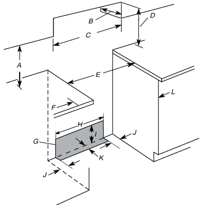
Freestanding Cutout
