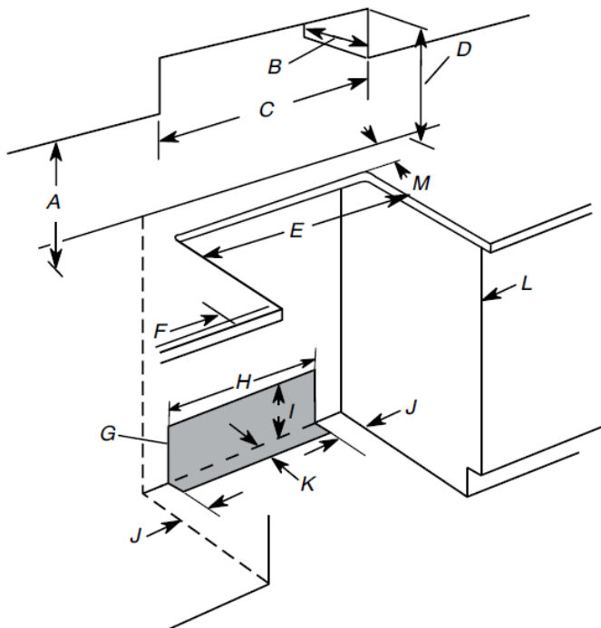
Slide-in Cutout
