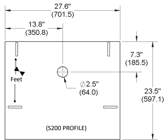
TOP DOWN VIEW OF COUNTER TOP
