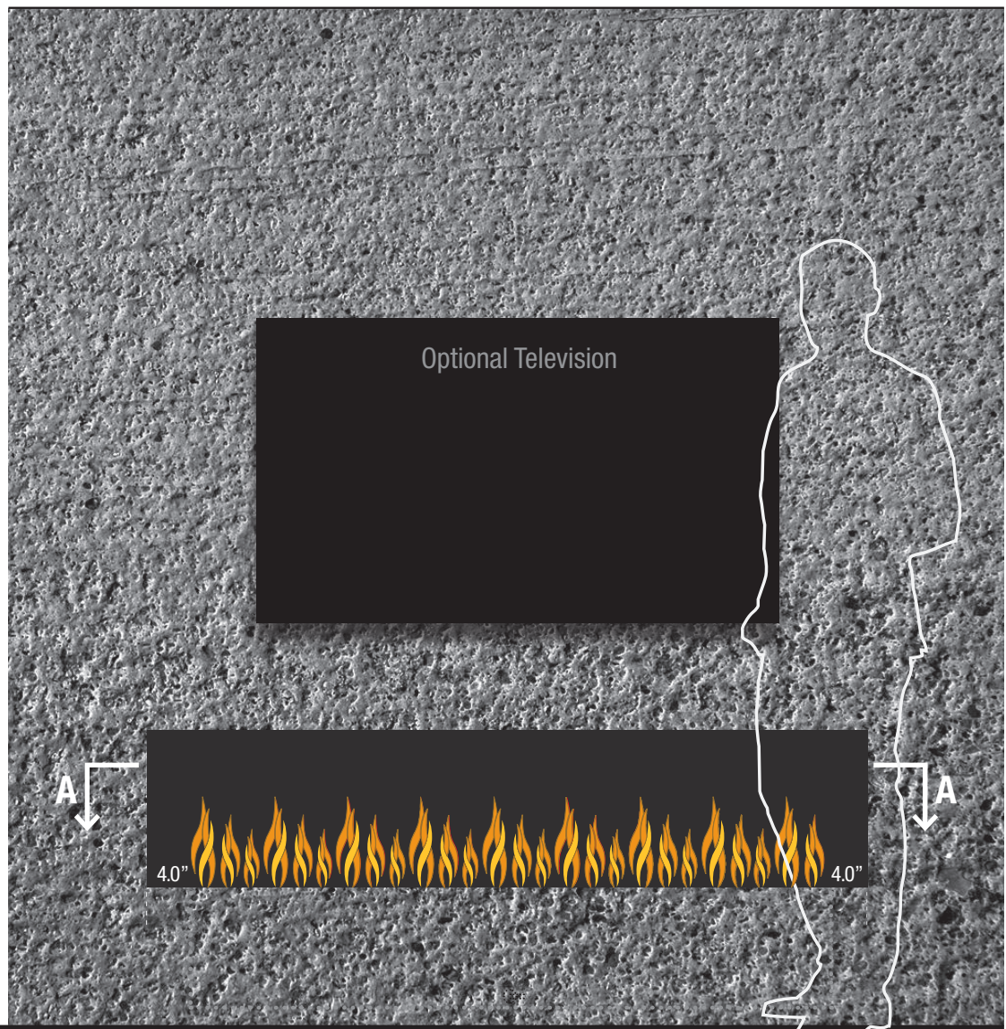
FRONT ELEVATION
