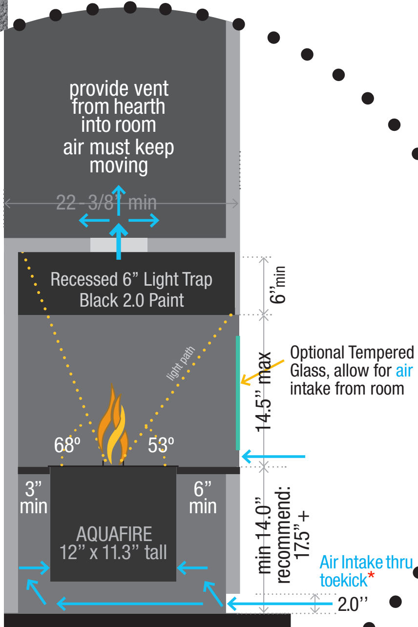
SIDE SECTION SCHEMATIC GLASS ENCLOSED RECESSED HEARTH
