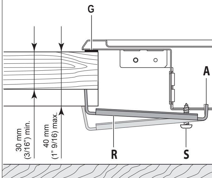
Rear Fixing Brackets
