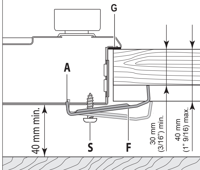
Front Fixing Brackets
