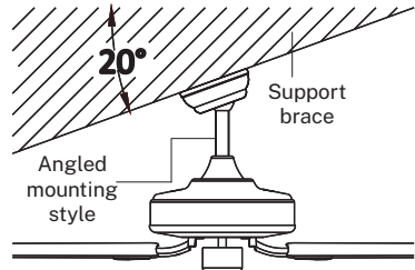
Angled Mounting recommended for a vaulted or angled ceiling.
