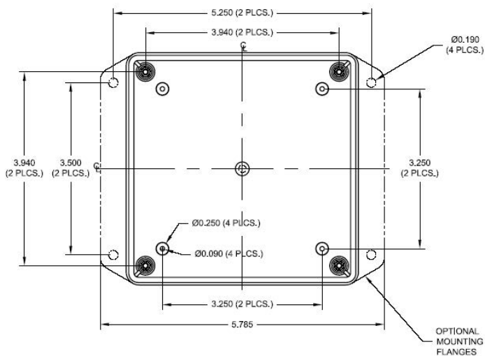
MRI Mounting Diagram (Figure 2)
