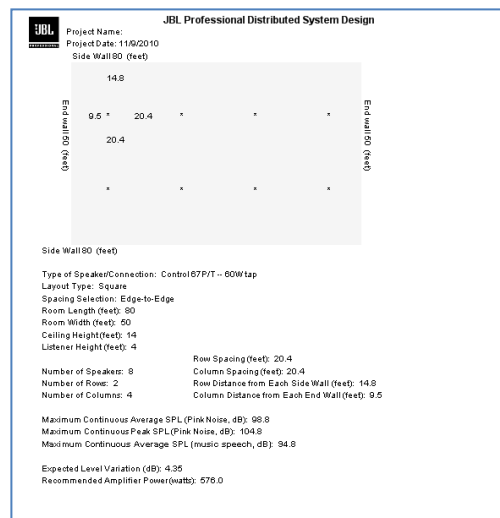
Design data from JBL's DSD Distributed Speaker Design Software
