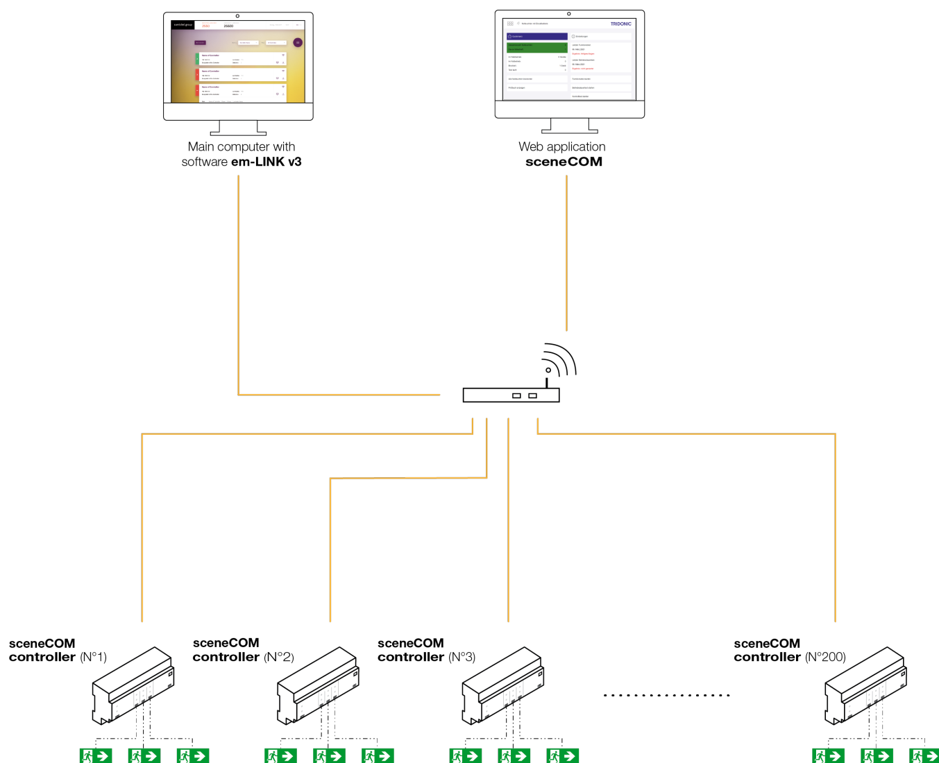
Figure 1: Topology
