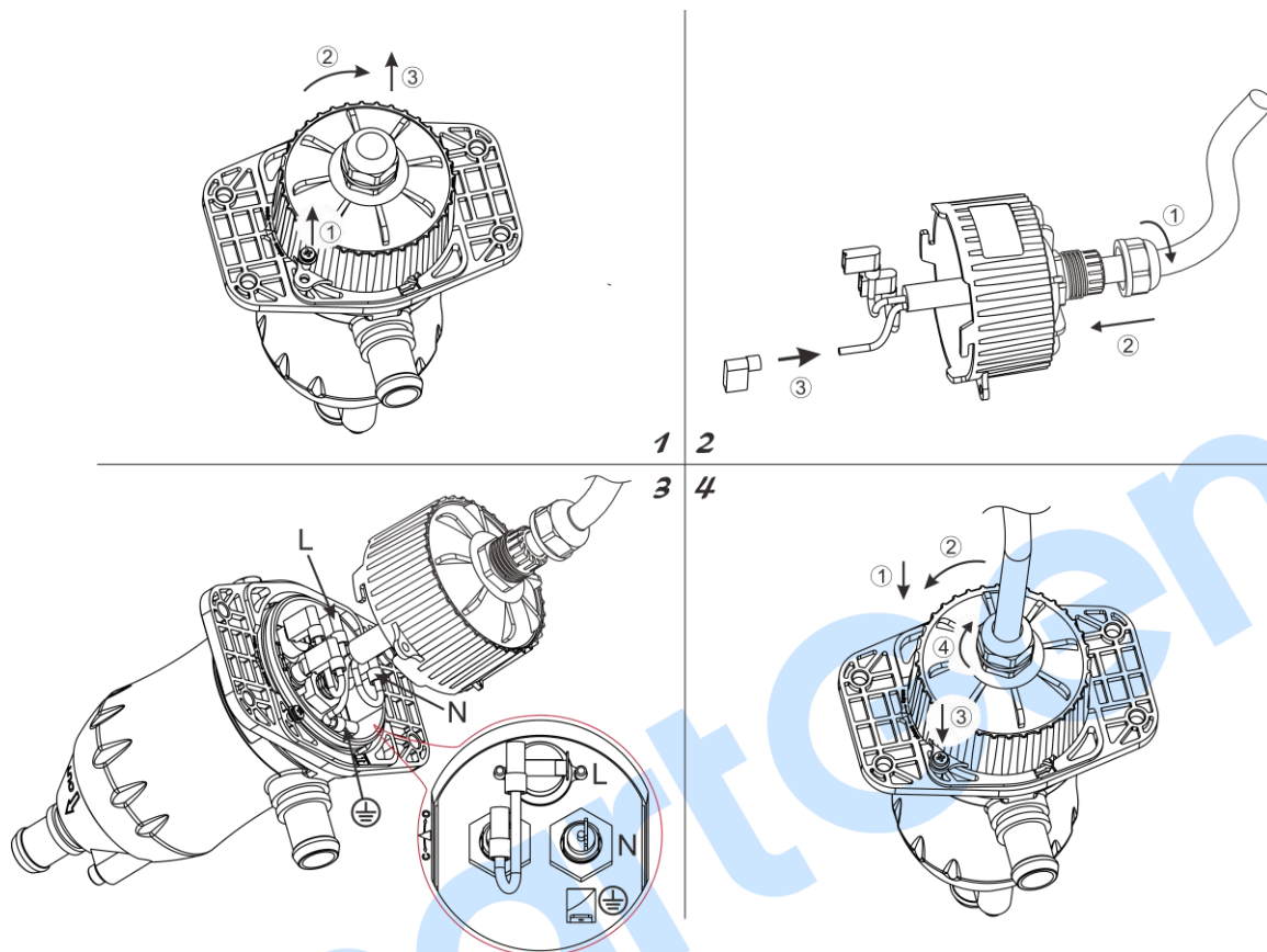
Fig.2 – Wiring Diagram
