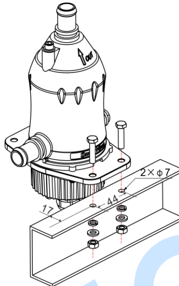
Fig.5 – Installation Diagram
