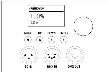
Figure 1 - Control Panel
