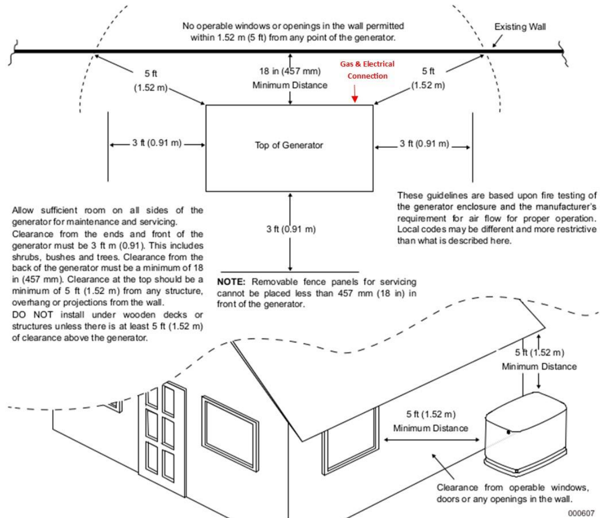
Figure 3-1. Installation Guidelines
