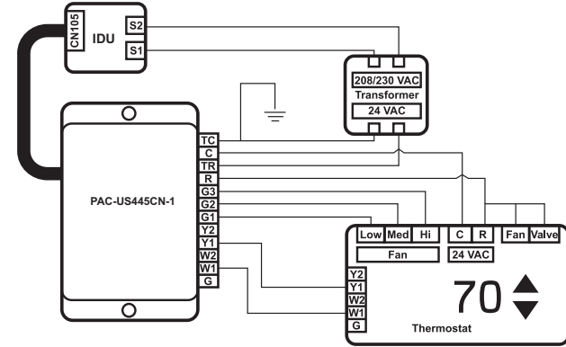
Example 4: Single-stage cooling with alternate primary heating source Note: For this configuration, it is recommended to set SW2-6 to the ON position. Follow the wiring from Example 2 with the following adjustments:
