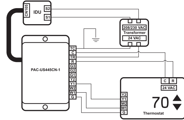
Example 2: Single-stage cooling and heating
