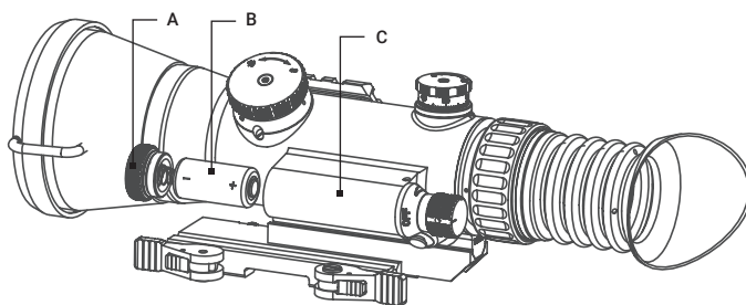
FIGURE 2-1. WOLVERINE 4 BATTERY INSTALLATION
