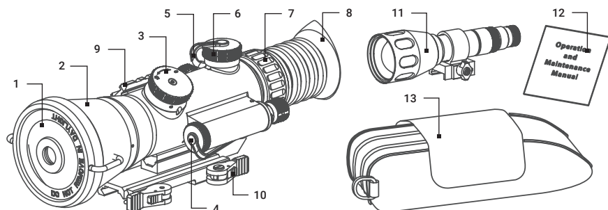
FIGURE A-1. WOLVERINE 4 SPARE PARTS
