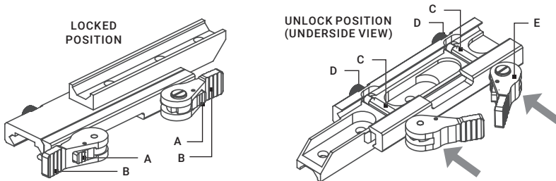
FIGURE 2-3. MOUNT
