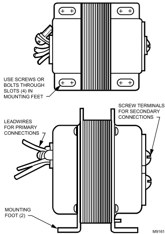
Fig. 1. Foot mounting.
