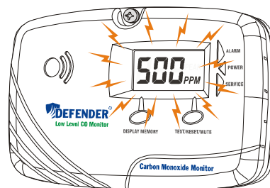
Display Flashes Above 500 PPM (e.g. 700 PPM detected)
