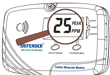
Highest CO Level (e.g. peak of 25 PPM detected since activated or cleared)
