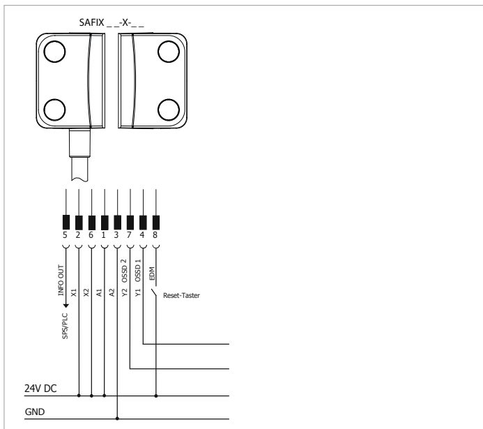
Figure 7: Input from a reset button Monitored for the EMD input variation (SAFIX __-X-__ ) The inputs X1 and X2 are supplied with 24 V DC. The outputs Y1 and Y2 are included in the analysis. The diagnosis output can be connected, for example, to an SPS. The input EDM waits for a start pulse duration between 30 ms and 5 s.
