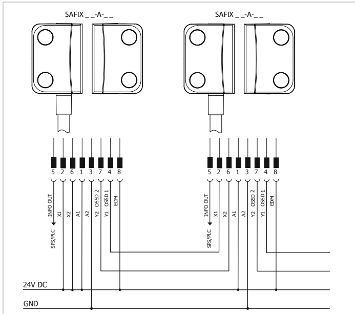
Figure 6: Series connection with diagnosis output, automatic reset Automatic for the EMD input variation (SAFIX __-A-__ ) The inputs X1 and X2 are supplied with 24 V DC. The outputs Y1 and Y2 are included in the analysis. The diagnosis output can be connected, for example, to an SPS.
