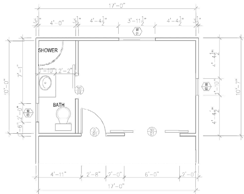
1 GROUND FLOOR PLAN Scale 1'=1/4"
