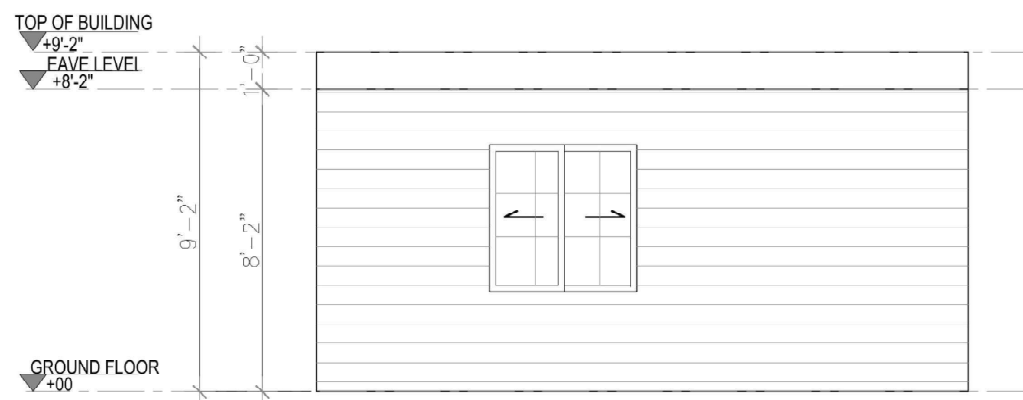
2 REAR ELEVATION Scale 1'=1/4"
