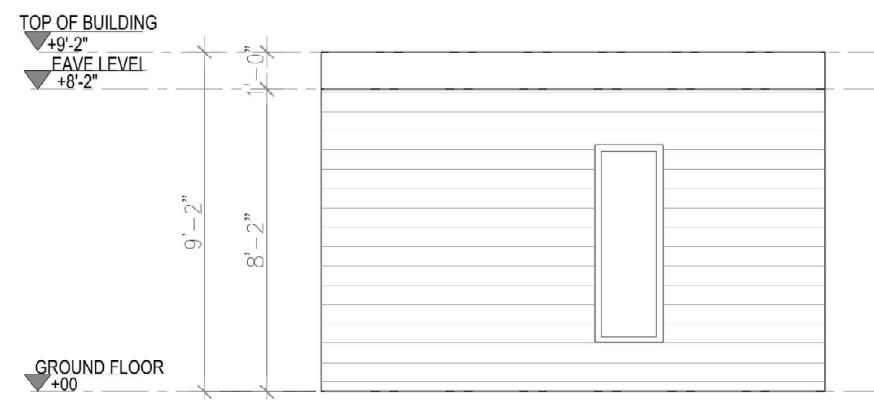
4 LEFT SIDE ELEVATION Scale 1'=1/4"
