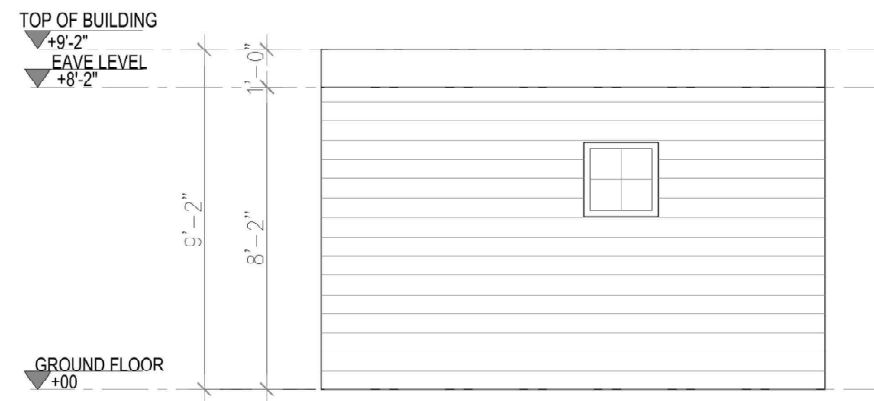
3 RIGHT SIDE ELEVATION Scale 1'=1/4"
