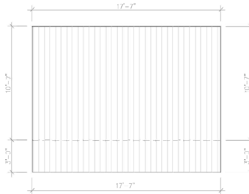
2 ROOF FLOOR PLAN Scale 1'=1/4"
