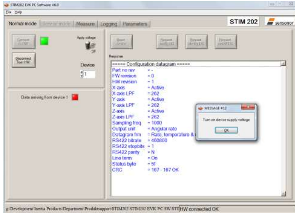
Figure 18: Normal mode panel when USB connector of STIM202 communication and power cable is to be inserted
