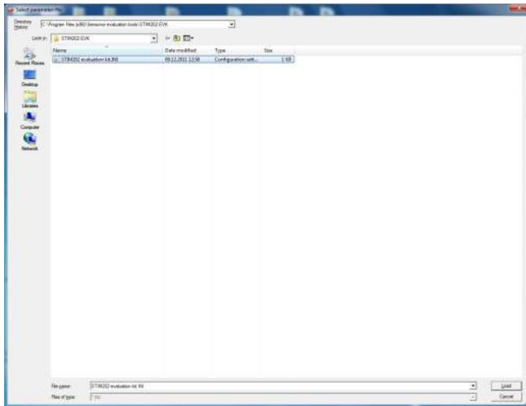
Figure 14: INI-file selection
