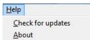
Figure 24: Help menu
