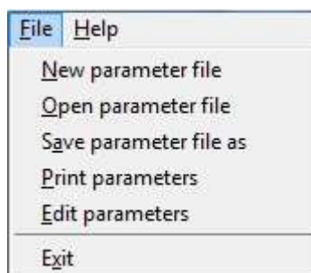
Figure 23: File Menu
