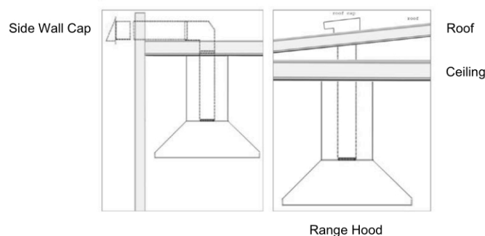
Option 1: Side Wall Venting
