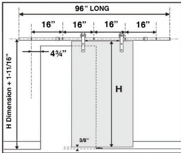
Suggested wall bracket spacing.
