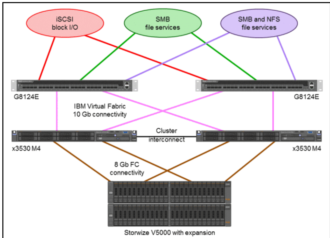
Figure 9. x3530 M4, Storwize V5000, and G8124E in the highly available unified gateway solution
