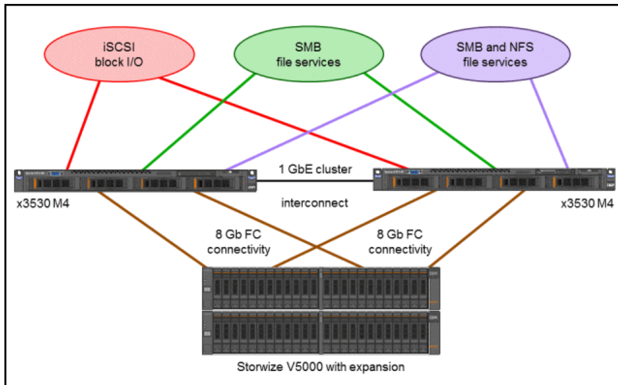
Figure 8. x3530 M4 and Storwize V5000 in a highly available unified gateway solution
